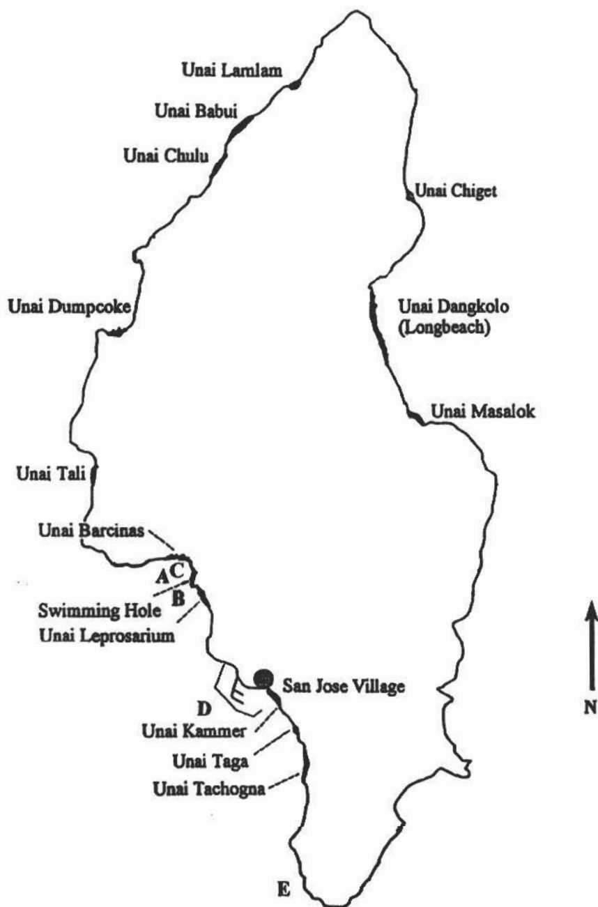
Figure 1. Island of Tinian with beaches indicated. Location of aquatic surveys: A) Two Corals/Barcinas Buoy, B) Swimming Hole, C) Barcinas, D) Harbor Wall, E) Carolinas Point.
