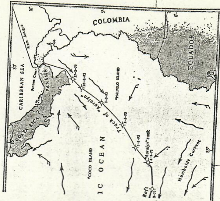
Here is shown the track of the raft together with the prevailing winds and currents experienced during the period of the year that the raft was in the area. The winds are shown by means of feathered arrows. The currents are shown by curly arrows.
