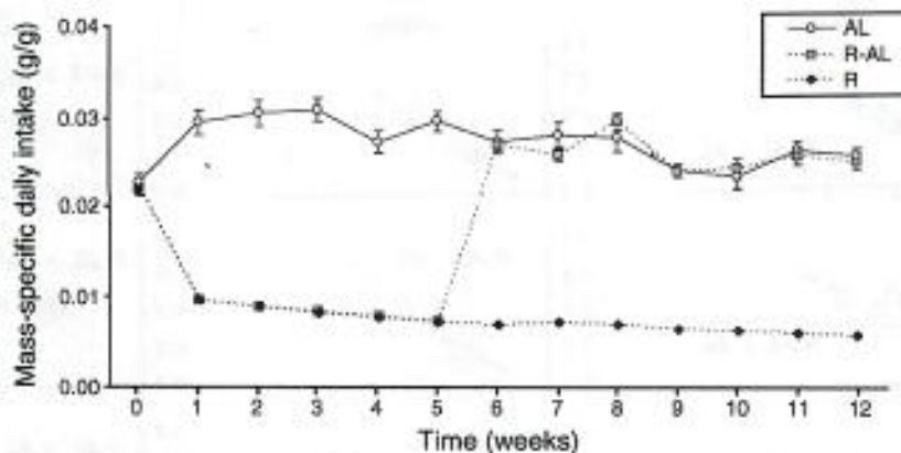
FIG. 3. Intake (mean \pm SE) in each week as a percentage of body mass. No significant differences were detected among AL and R-AL turtles after the diet switch at the beginning of week 6. Sample sizes and treatment groups are as in Fig. 1.
