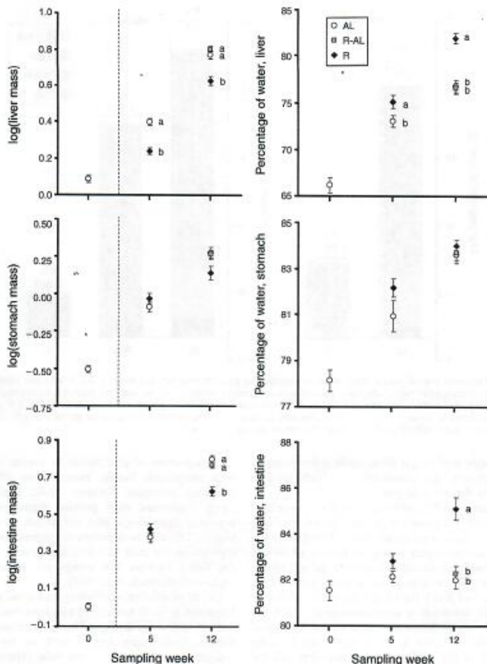
FIG. 4. Wet mass (left panels) and water content (right panels) of liver, stomach, and intestine from turtles at the end of weeks 0, 5, and 12 (mean \pm SE). The dashed line in the left panels separates actual values in week 0 from estimated marginal means in weeks 5 and 12. For organ masses, different letters associated with data points indicate values that are significantly different ( P < 0.05 ) within weeks according to ANCOVA [covariate = \log(\text{body mass excluding gut contents}) ] with a Bonferroni correction for multiple comparisons. For water content, different letters associated with data points indicate values that are significantly different ( P < 0.05 ) within weeks according to ANOVA and Tukey's h sd post hoc test. Sample sizes: n = 10 turtles per group at each time point. Treatment groups are as in Fig. 1.
