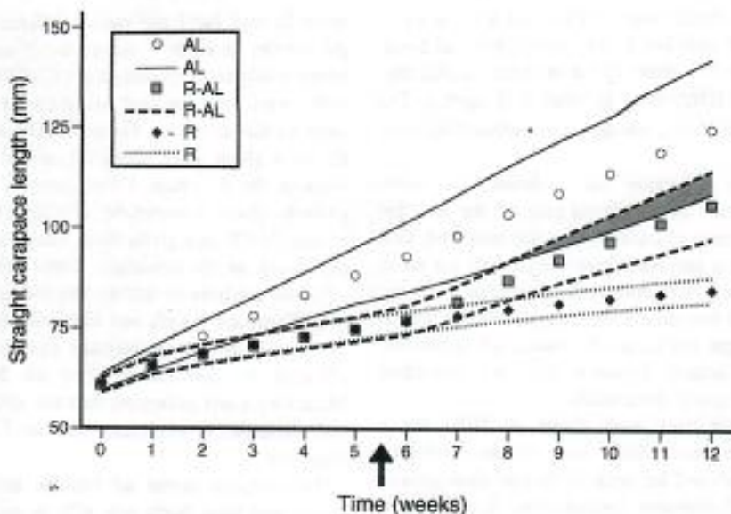
FIG. 1. Straight carapace length at the midpoint of each week for juvenile green turtles ( Chelonia mydas ) in three treatment groups: AL, ad libitum for 12 weeks; R, food-restricted for 12 weeks; R-AL, food-restricted for five weeks and ad libitum for seven weeks. The arrow indicates when R-AL turtles were switched from a restricted to an ad libitum diet. Points represent means, lines represent \pm SD from the mean, and the shaded area is the region of overlap in standard deviations of AL and R-AL turtles. Sample sizes: n = 37 AL, 39 R-AL, and 39 R turtles (weeks 0–5); n = 17 AL, 29 R-AL, and 29 R turtles (weeks 6–12).
