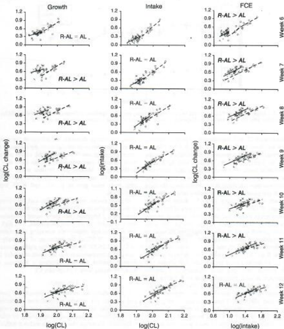
FIG. 2. Regressions for growth, intake, and food conversion efficiency (FCE) in AL (open circles, dashed lines) and R-AL (crosses, solid lines) juvenile green turtles in each of weeks 6–12, when both groups were feeding ad libitum. Data were log-transformed prior to analysis to satisfy the assumptions of ANCOVA. CL indicates straight carapace length; treatment groups are as in Fig. 1. The equation in each graph refers to ANCOVA results; boldface indicates P < 0.05 ; italicized boldface indicates P < 0.01 . The log-transformed dependent variables were change in CL (for growth and FCE) and average daily intake \times 7 (for intake). The log-transformed covariates were CL at the beginning of the week (for growth), CL at the middle of the week (for intake), and average daily intake \times 7 (for FCE). A comparison of intake in AL and R-AL turtles in week 6 was not possible because of a significant treatment \times covariate interaction. Sample sizes: n = 17 AL and 29 R-AL in each week.
