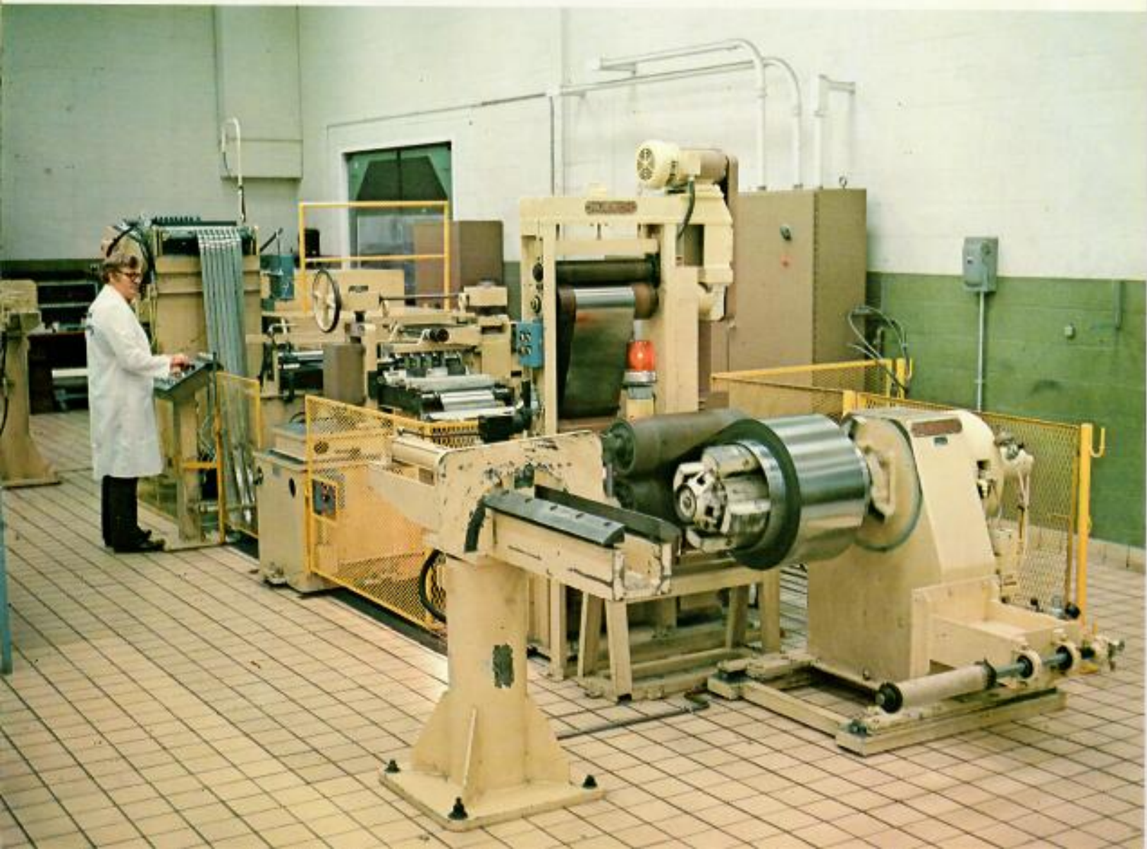
Below: Slitting line with X-Ray thickness gauge.
