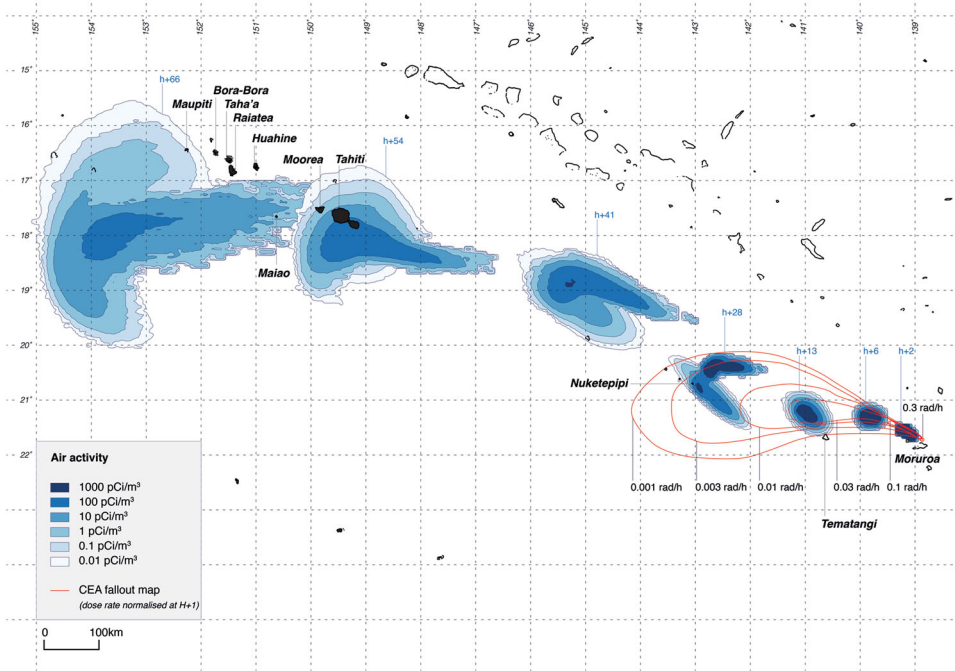
Figure 2. Reconstruction of the 1974 Centaure cloud trajectory over French Polynesia. Air activities in \text{pCi/m}^3 ( 1 \text{ pCi} = 0.037 \text{ Bq} ) between 0 and 500 m were obtained using the HYSPLIT atmospheric transport code (see Appendix A ).
