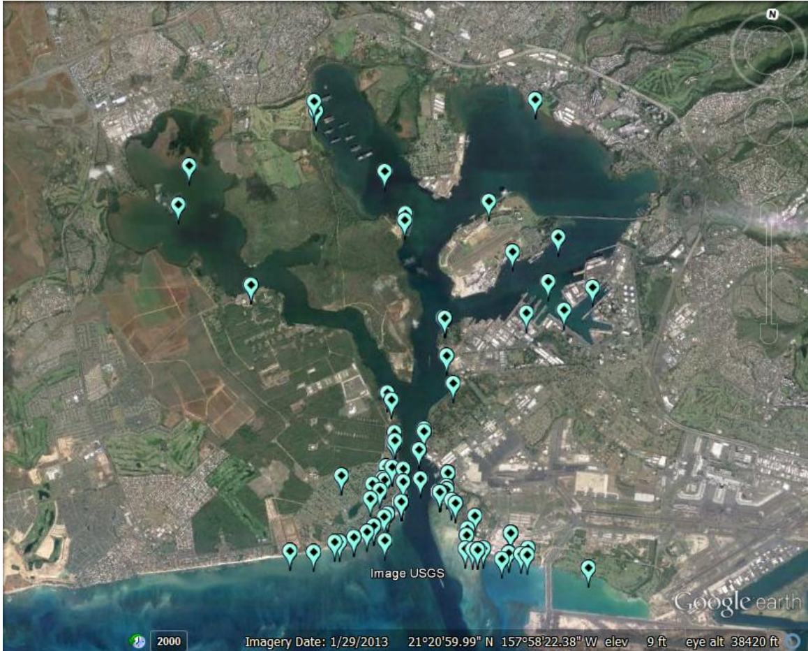
Figure 1: Locations of each marine turtle which stranded in Pearl Harbor and adjacent areas are mapped to show the exact locations of each event. Of the total stranding events (n=184), 177 cases included GPS points and are mapped.
