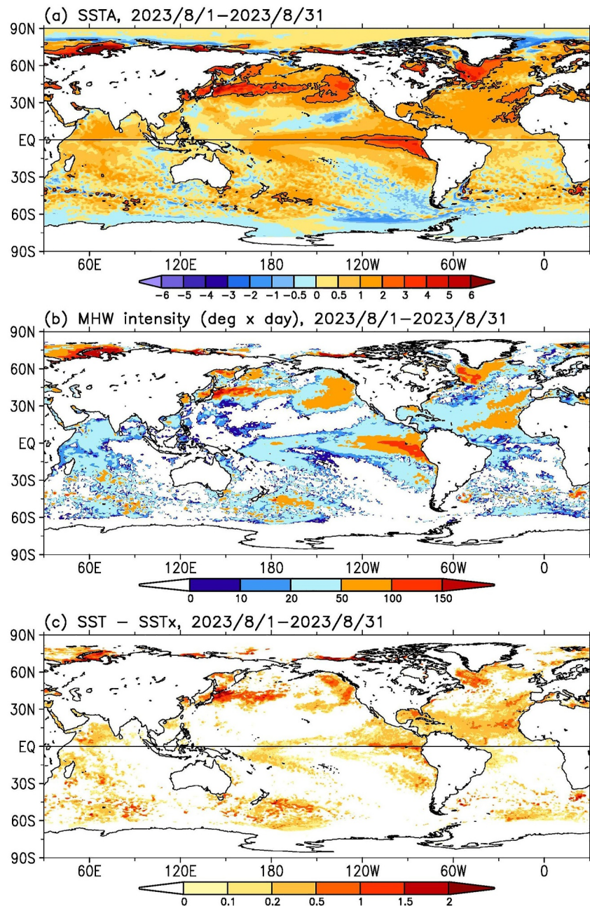
Figure 2. Record-high SSTAs in August 2023 expressed in (a) average SSTAs ( ^{\circ}\text{C} ), (b) conventional MHW intensity index (degree-day), and (c) super-MHW intensity ( ^{\circ}\text{C} ).
