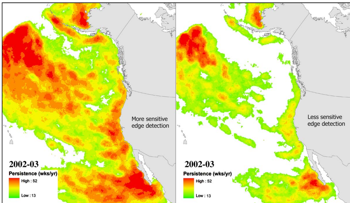
Fig. 6. A comparison of persistence values for high densities of temperature fronts in the Northeast Pacific using a sensitive edge-detection algorithm (left—slope 0.015\% ) and a strict edge detection algorithm (right—slope 0.020\% ) in NAVOCEANO 18-km interpolated SST.
