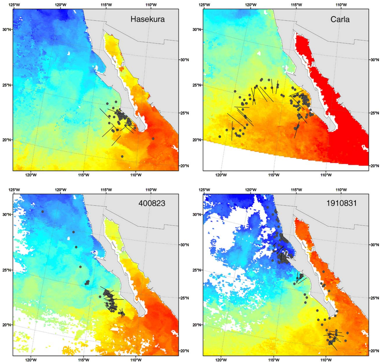
Fig. 2. Four examples of the virtual transects used to identify biologically relevant SST gradient transects across sea turtle and blue whale trajectories in 9 km weekly (8 day) AVHRR.
